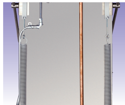
Two heavy springs on the back of the unit counterbalance the easy-lift four-sided door.
