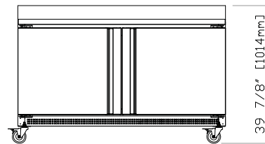
FWR(F)-60 Front View
