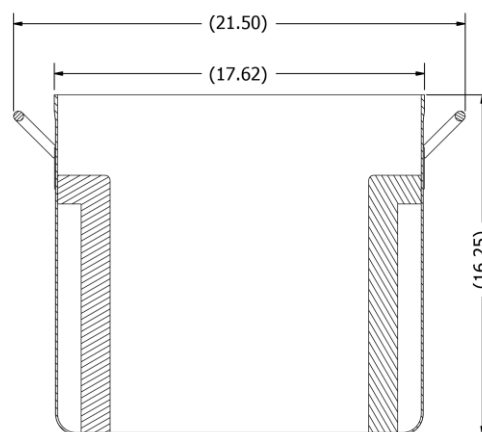
2707M Cross Section Dimension View
