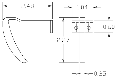
SIDE BLADE (2 EA)
