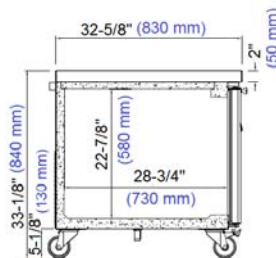
RIGHT VIEW
