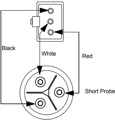
Ohm water Level Probe and Wiring Harness
