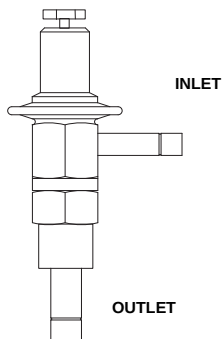
HPR VALVE
